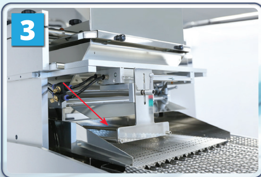
3 The Adjustable Variable Speed Diverter Bar Above the Product Channels, Sweeps Left & Right to Eliminate "Twinning"
