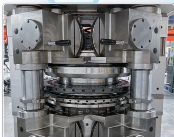
Servo Control for Compression Rollers
