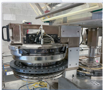
Easy Turret Removal
