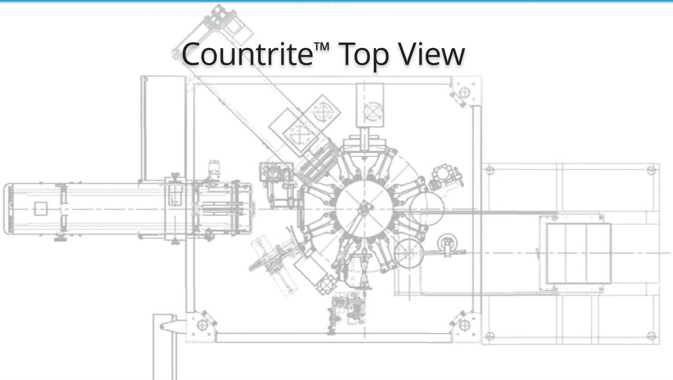
CountRite™ – 8 Station Pre-made Gusseted Bag Counting System
