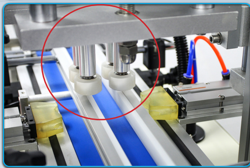
Four Cap Tightening Spindles
