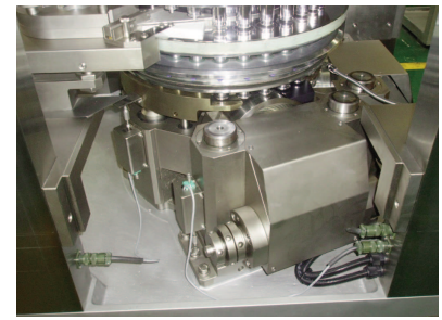
PRE-COMPRESSION LOWER
