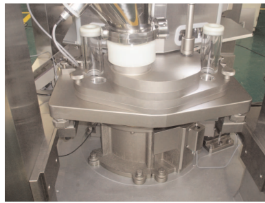
MECHANICAL FEEDER
