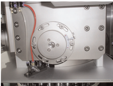
MAIN COMPRESSION UPPER DIAL WITH JET SPRAY LUBRICATION CONTROL
